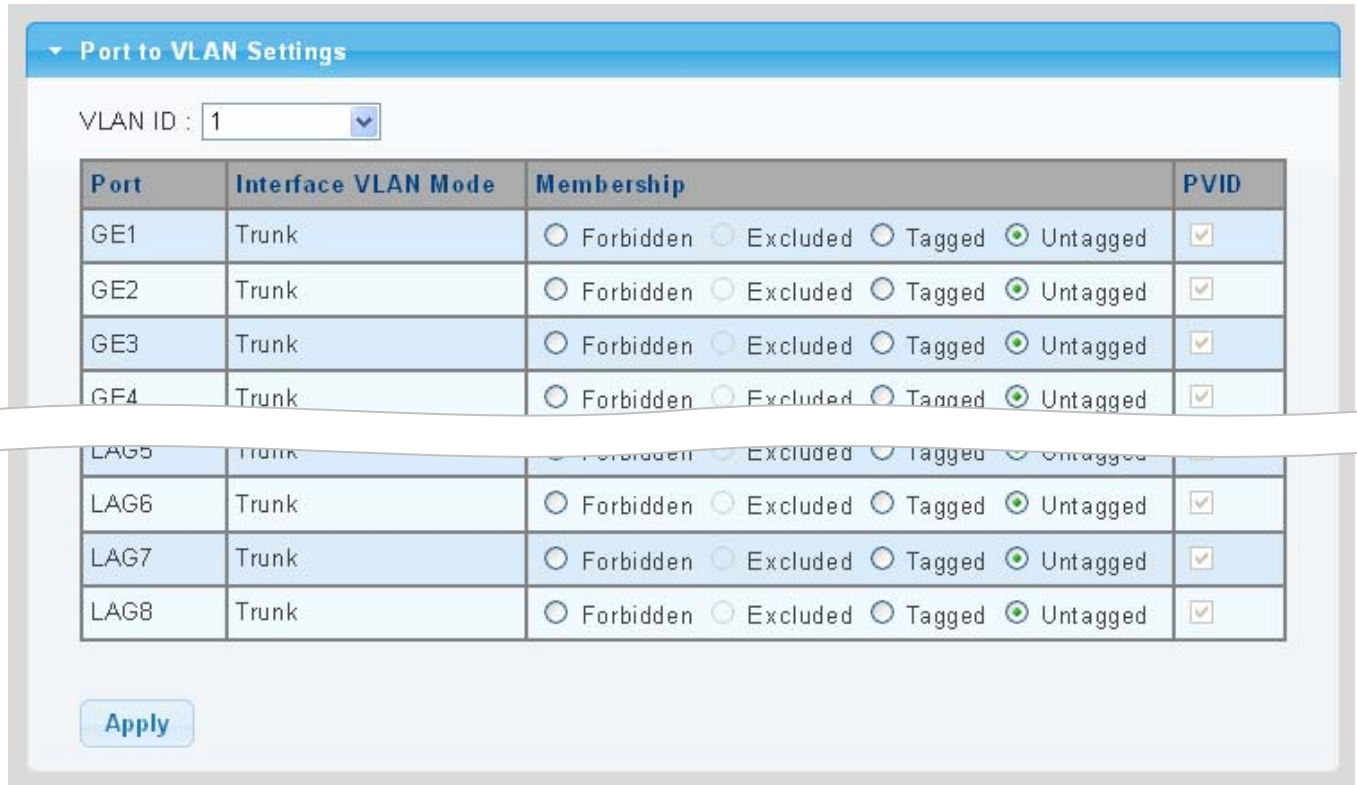
Figure 4-5-7 Port to VLAN Setting Page Screenshot
