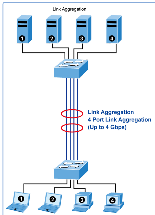
Figure 4-4-1 Link Aggregation
