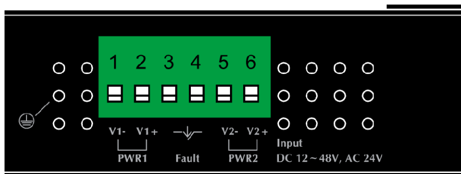
Figure 2-3: IGS-801M Upper Panel
