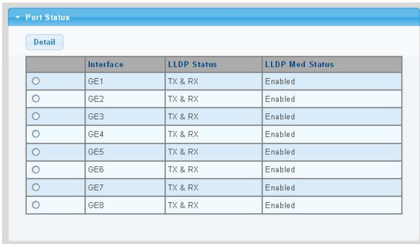
Figure 4-12-8 Port Status Page Screenshot
