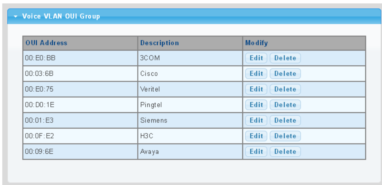
Figure 4-8-25 Voice VLAN OUI Group Page Screenshot
