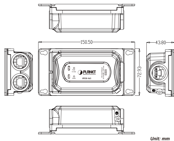
Figure 2-1: IPOE-165 product outlook
