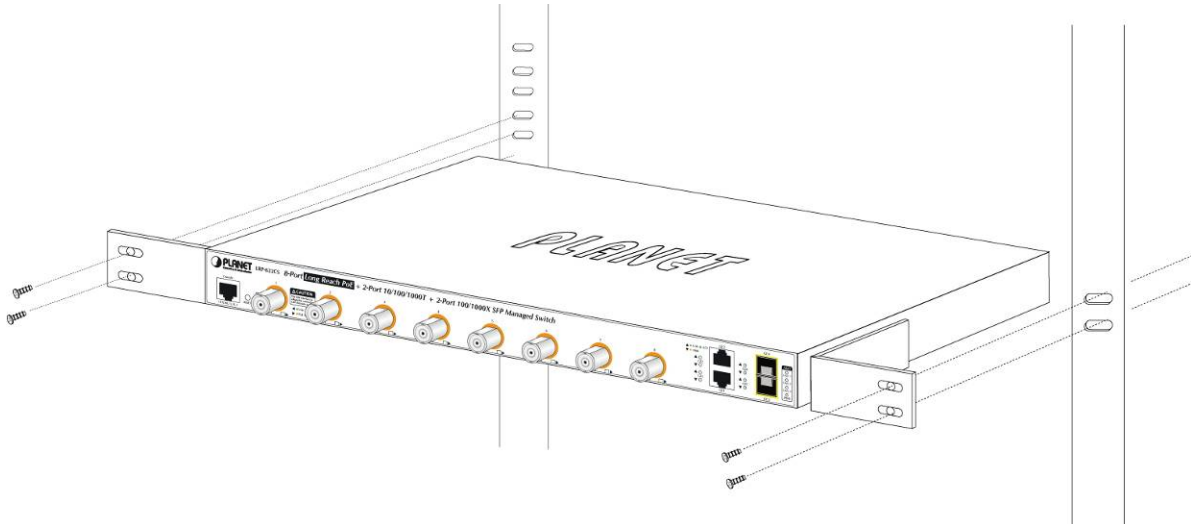
Figure 2-1-6 Mounting LRP Managed Switch in a Rack
