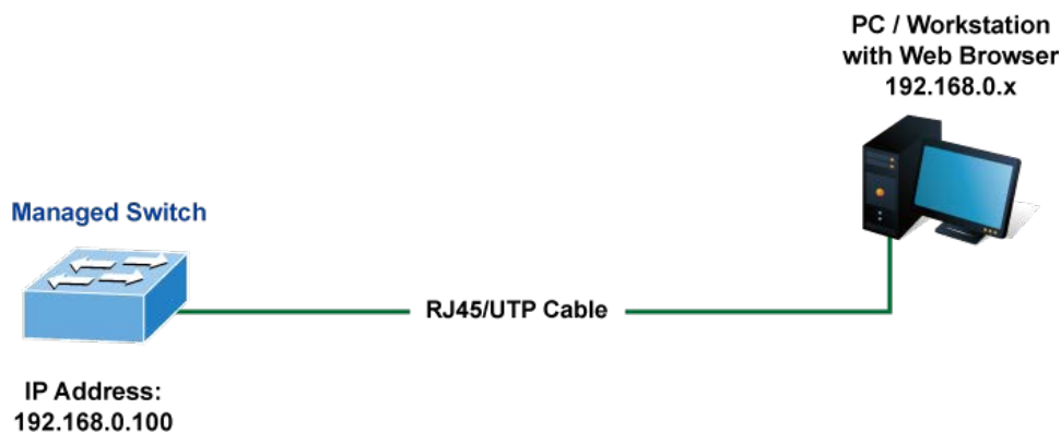
Figure 4-1-1 Web Management
