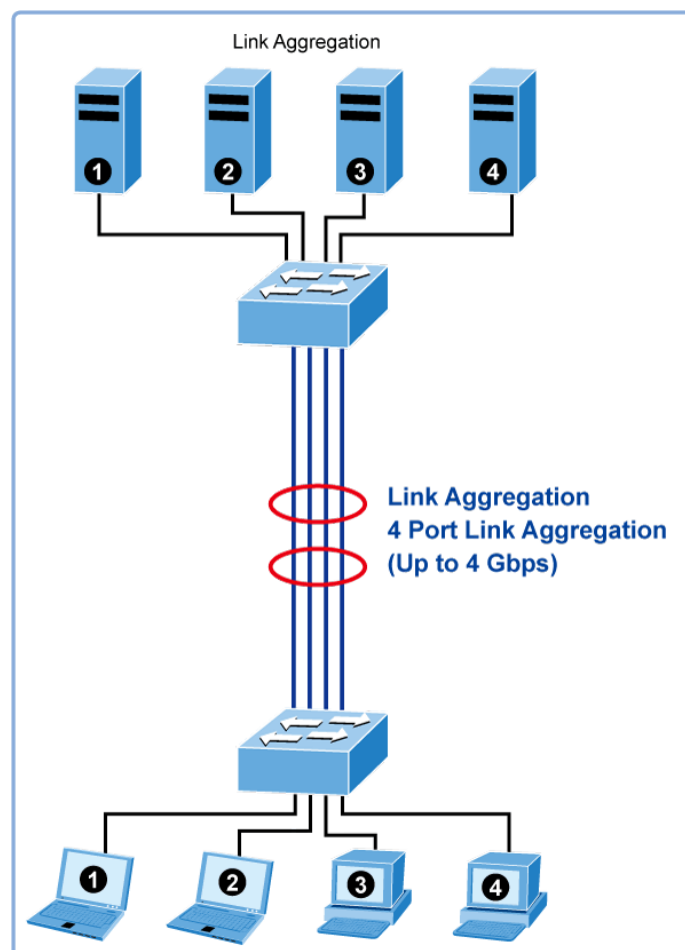
Figure 4-4-1 Link Aggregation
