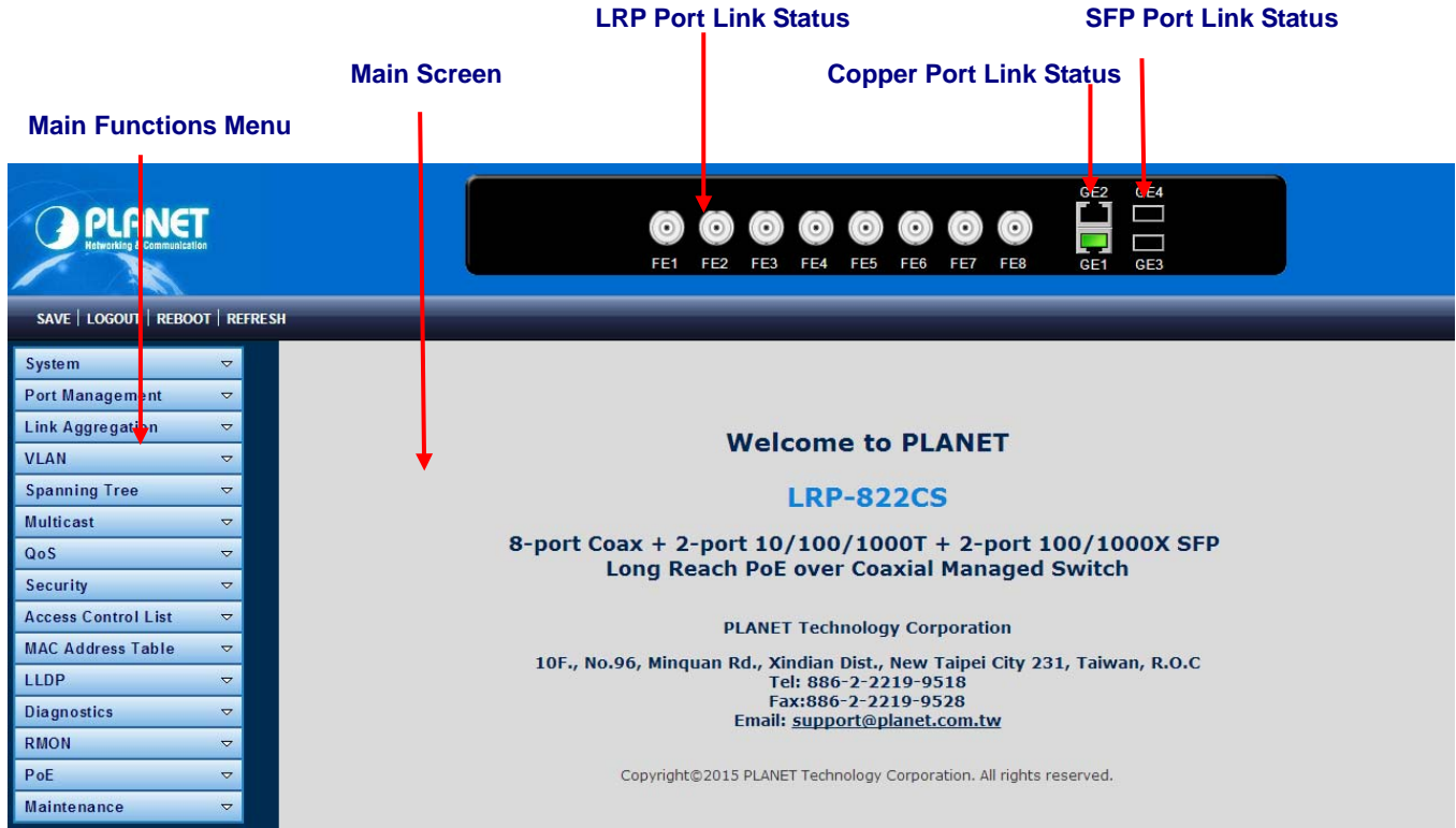
Figure 4-1-4 Main Page
