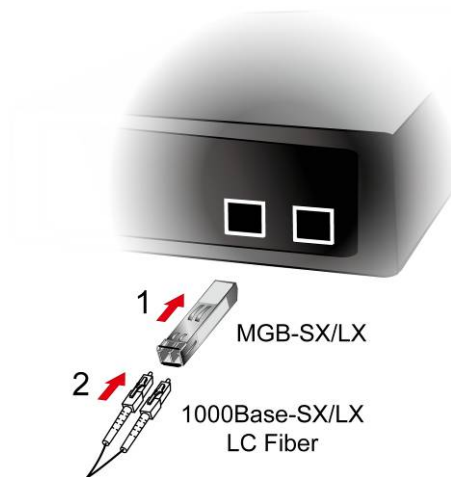
Figure 2-1-7 Plug in the SFP transceiver
