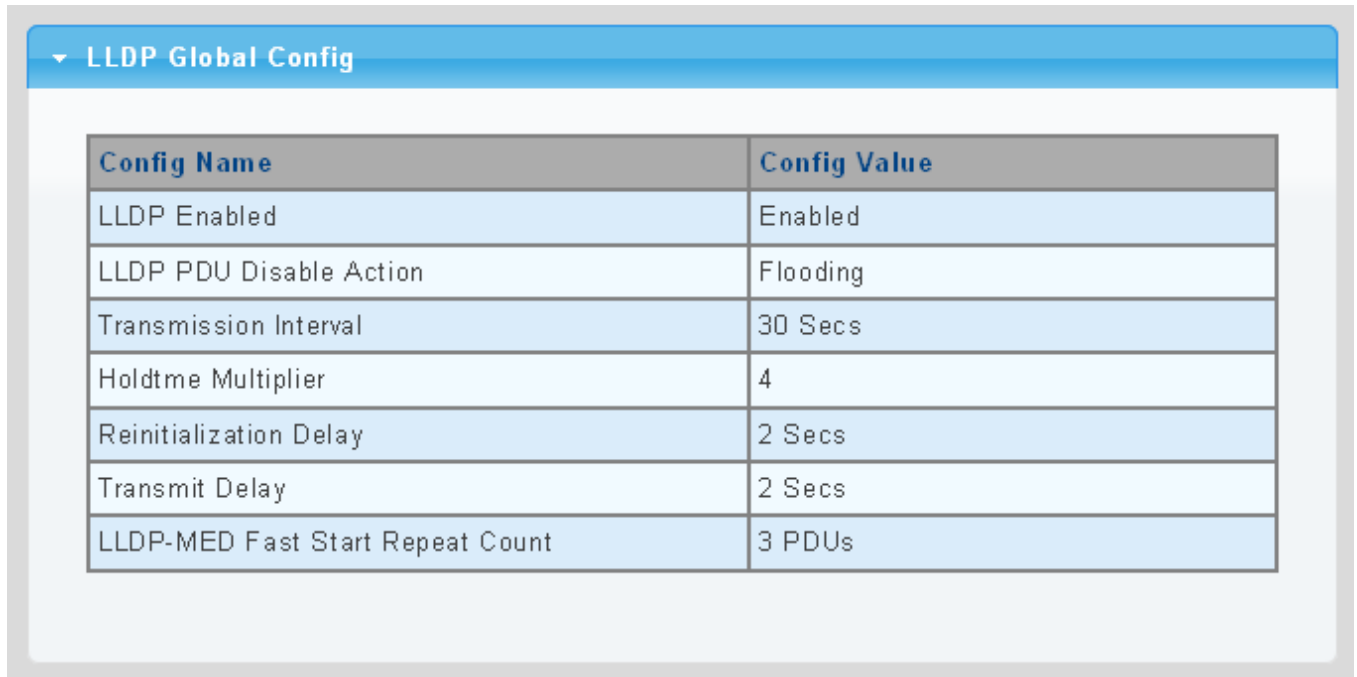
Figure 4-12-2 LLDP Global Config Page Screenshot
