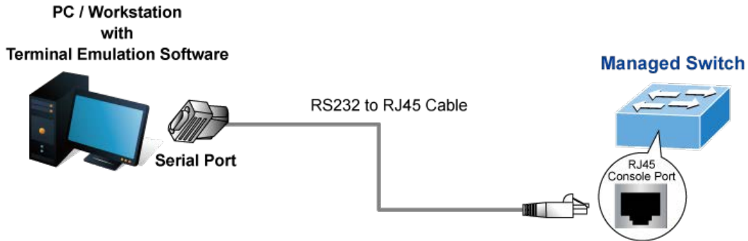
Figure 3-1-1: Console Management
