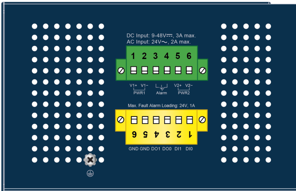
Figure 2-1-4e: Upper Panel of IGS-4215-24T4X
