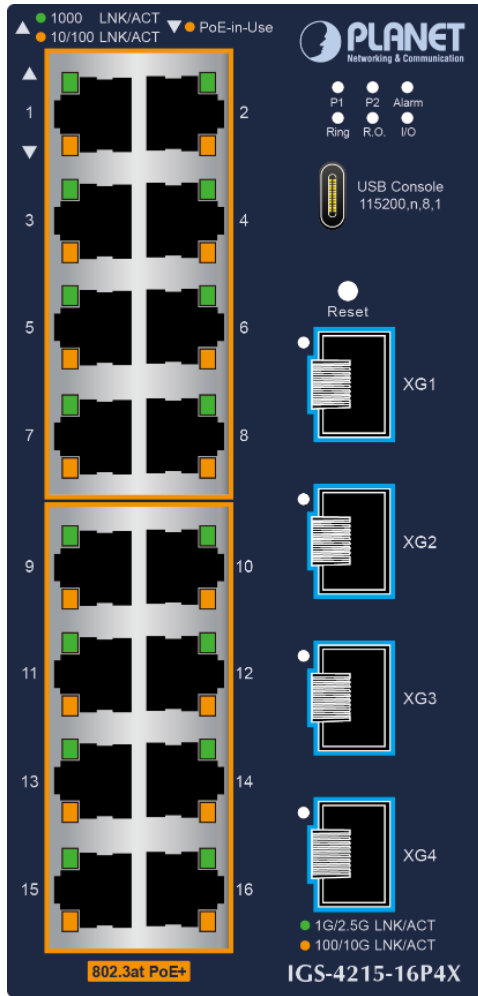
Figure 2-1-3d: IGS-4215-16P4X
