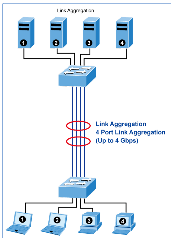
Figure 4-4-1: Link Aggregation
