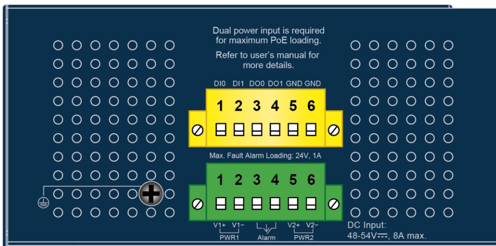
Figure 2-1-4b: Upper Panel of IGS-4215-8UP4X
