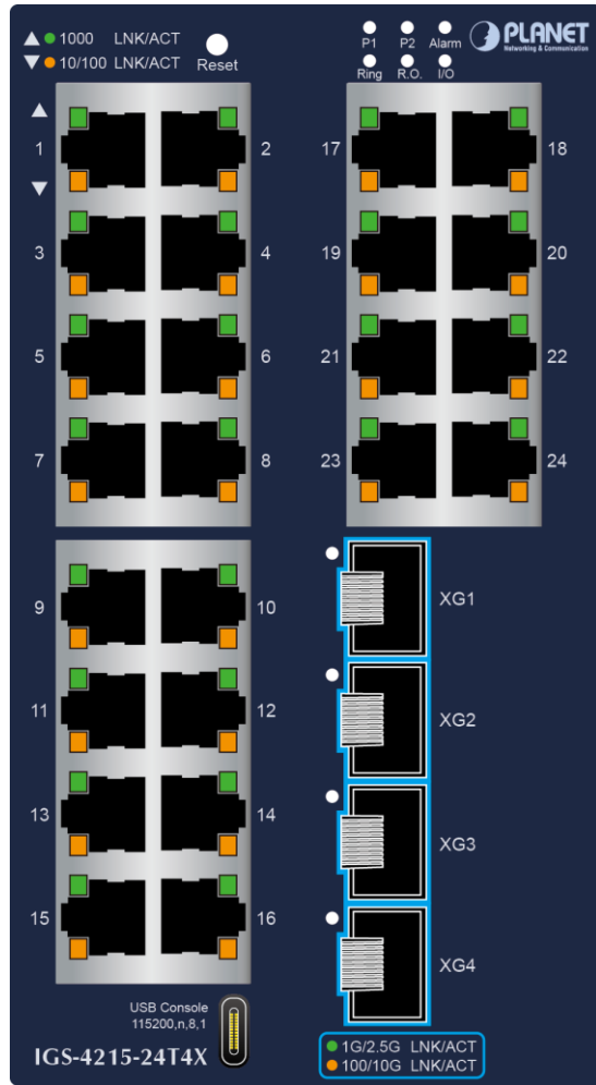
Figure 2-1-3e: IGS-4215-24T4X
