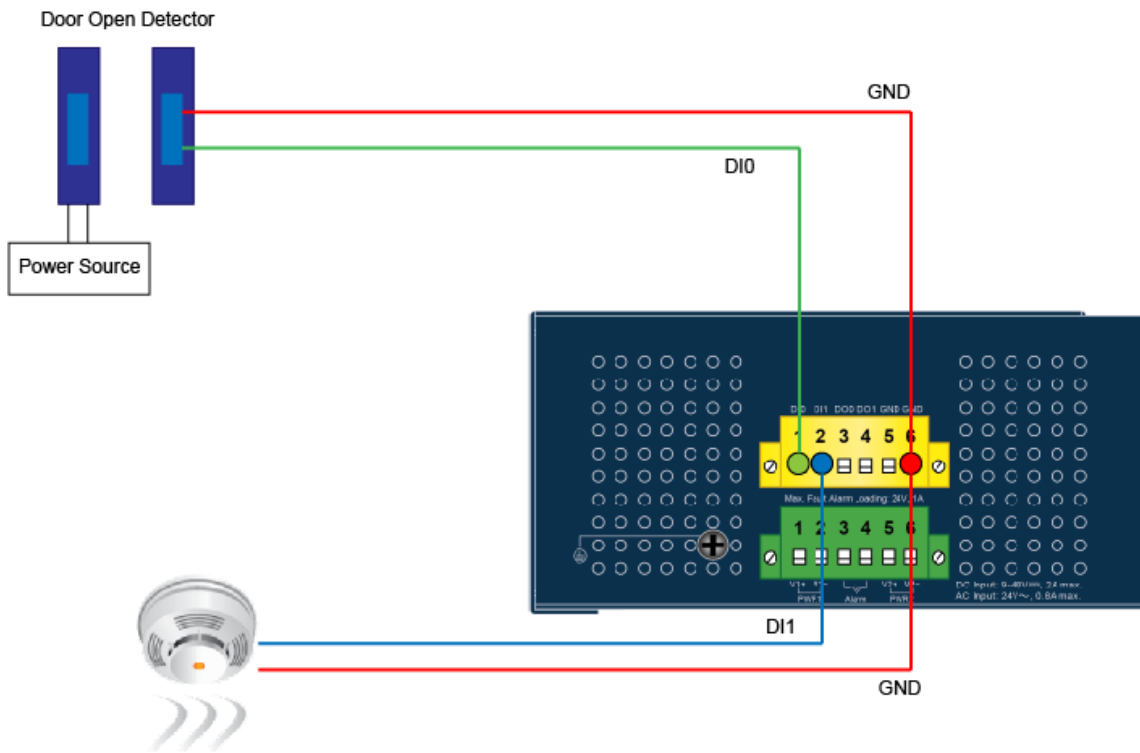
Figure 2-1-7c Wiring DIO and DI1 to Open Detector
