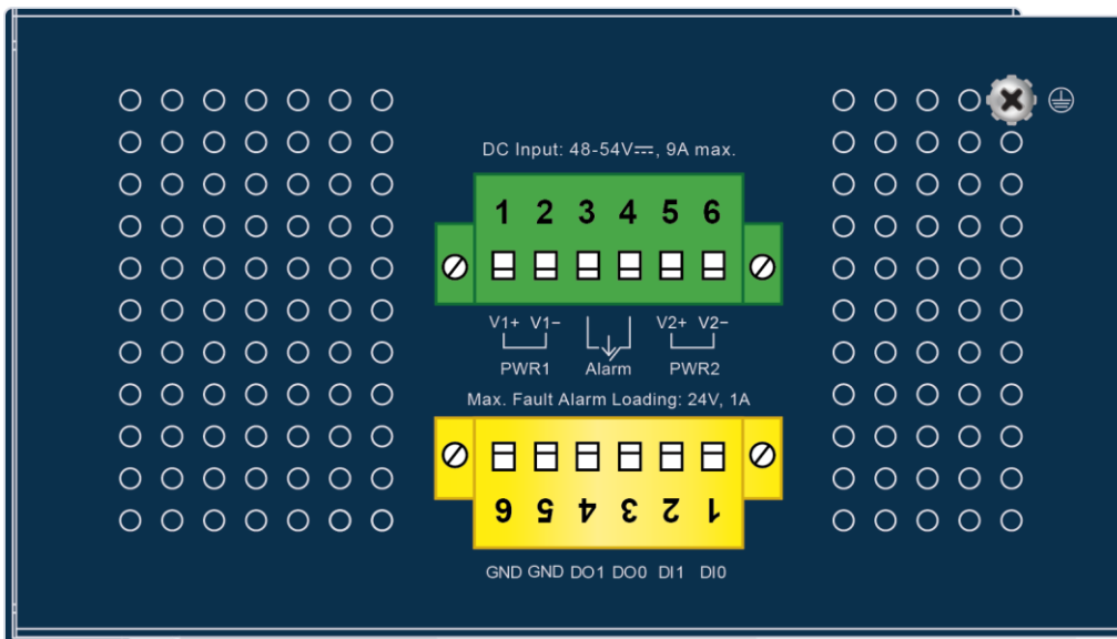
Figure 2-1-4d: Upper Panel of IGS-4215-16P4X
