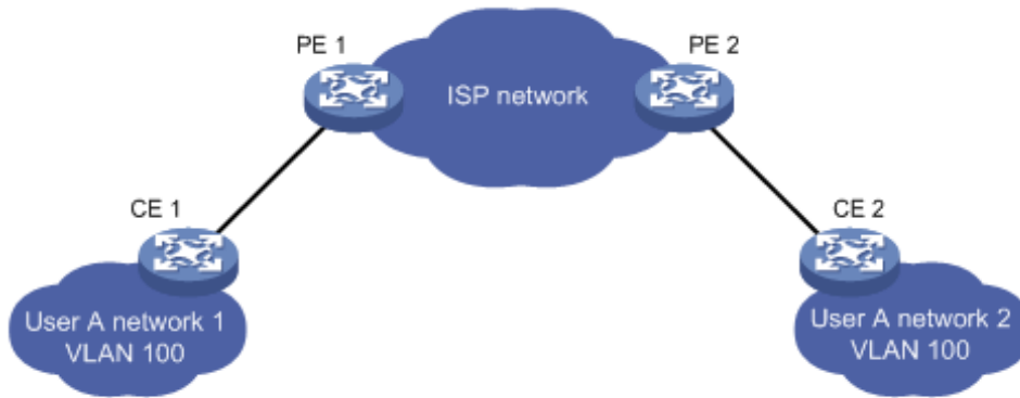
Fig 8-1 BPDUs Tunnel application
