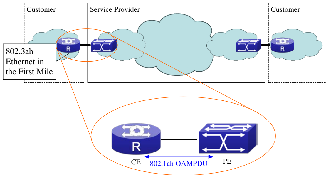
Fig 10-2 Typical OAM application topology
