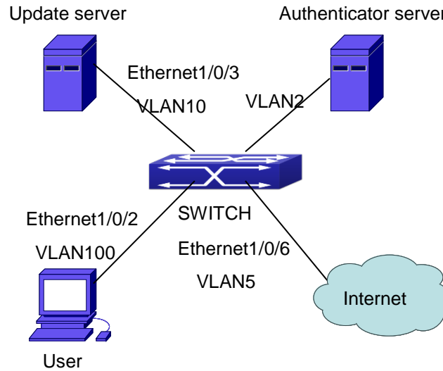
Fig 3-13 The Network Topology of Guest VLAN
