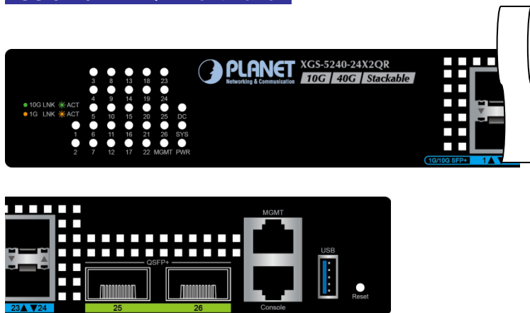
Figure 2-1-2 XGS-5240-24X2QR LED panel
