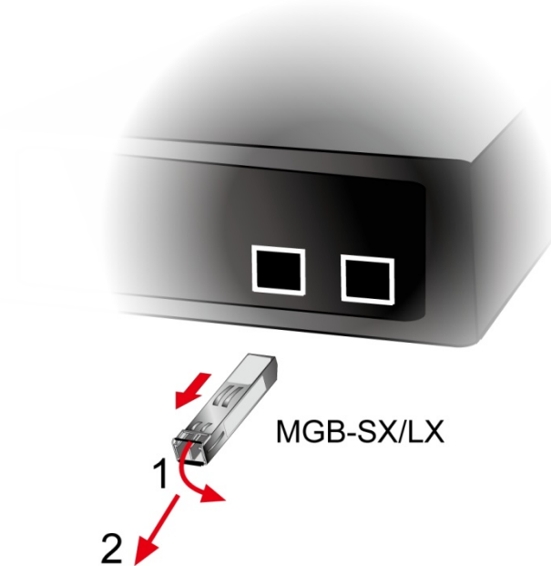
Figure 2-17: How to Pull Out the SFP/SFP+ Transceiver
