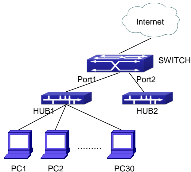
Fig 5-1 a typical configuration example of AM function
