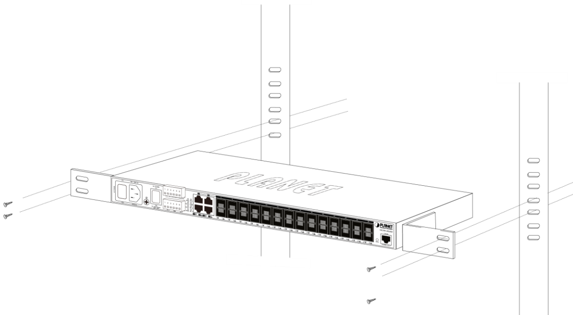
Figure 2-2-2-1 Mounting the Managed Switch on a Rack
