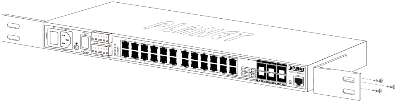
Figure 2-2-2-1 Attach Brackets to the Managed Switch.
