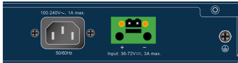
Figure 2-1-4-1: GS-5220-16S8CR AC inlet power socket
