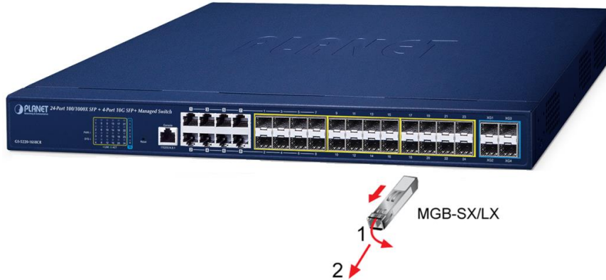
Figure 2-3-2-1: Pull out the SFP Transceiver Module
