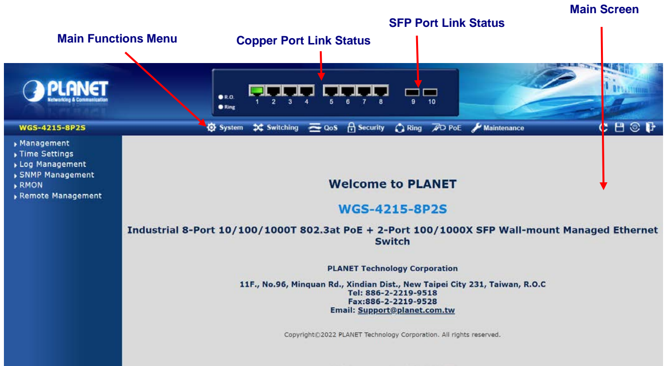
Figure 4-1-4 Main Page
