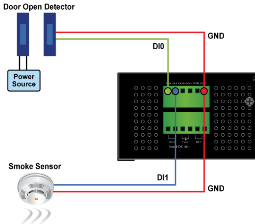
Figure 2-1-7c Wiring DI0 and DI1 to Open Detector
