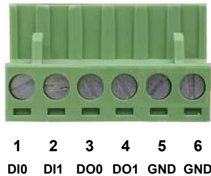
Figure 2-1-7b 6-pin Terminal Block for DI and DO Wiring Input
