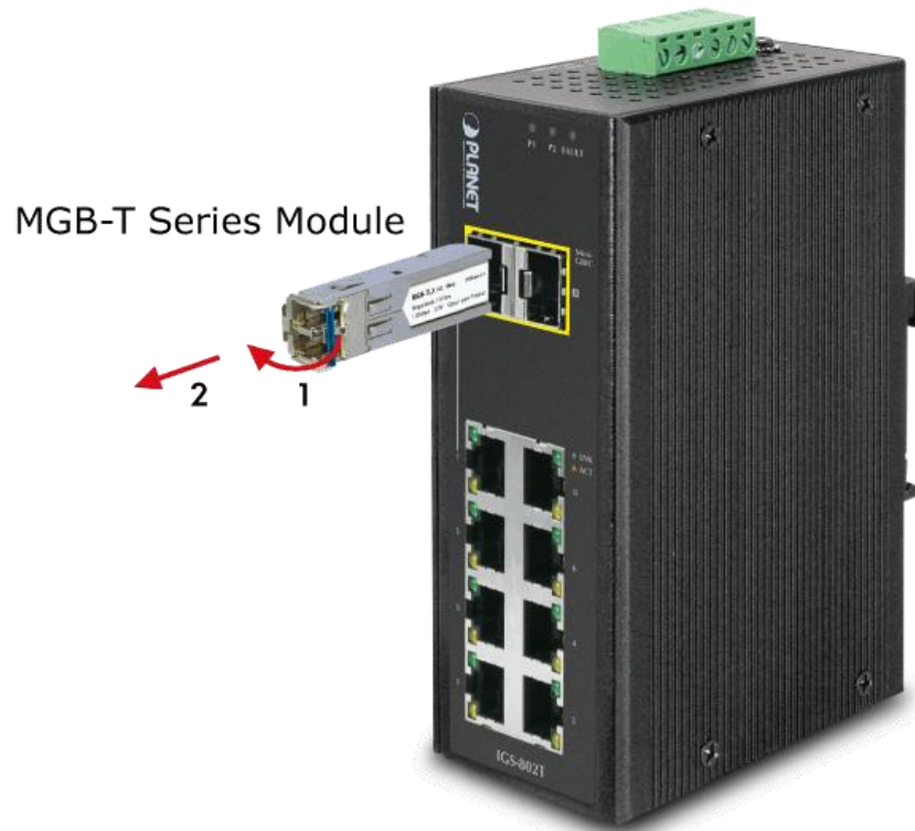
Figure 2-2-5: Pulling out the SFP Transceiver Module
