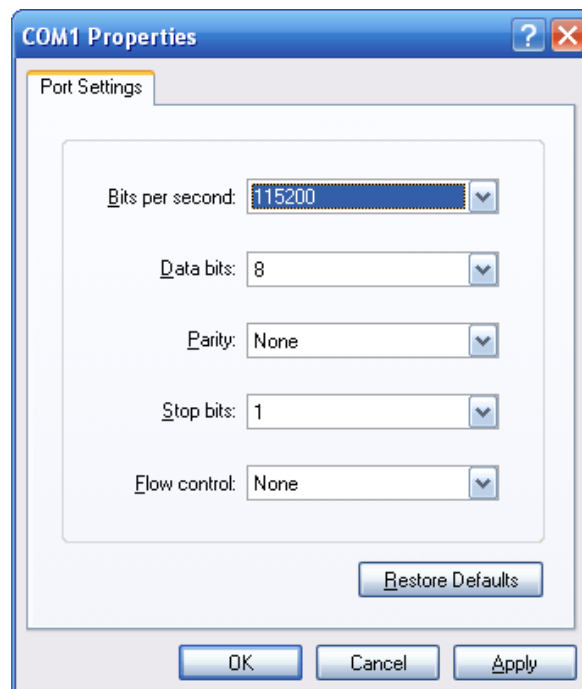
Figure 3-1-2: Terminal Parameter Settings
