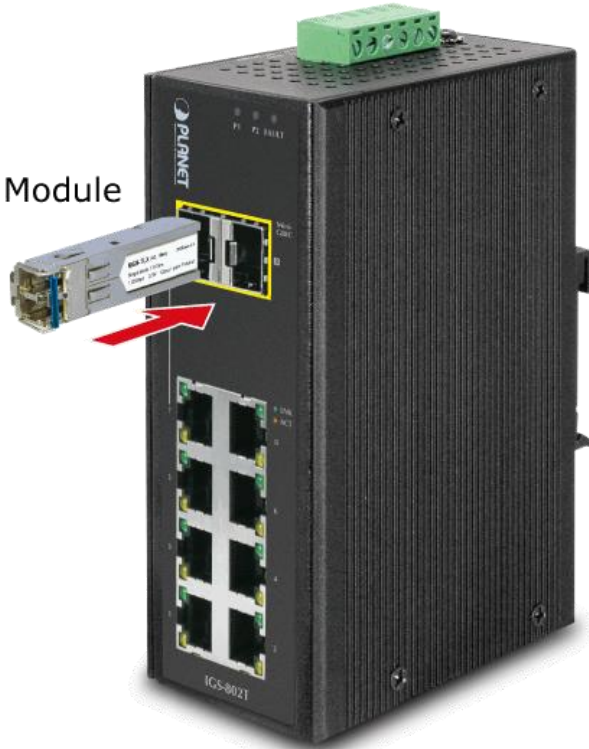
Figure 2-2-4: Plugging in the SFP Transceiver
