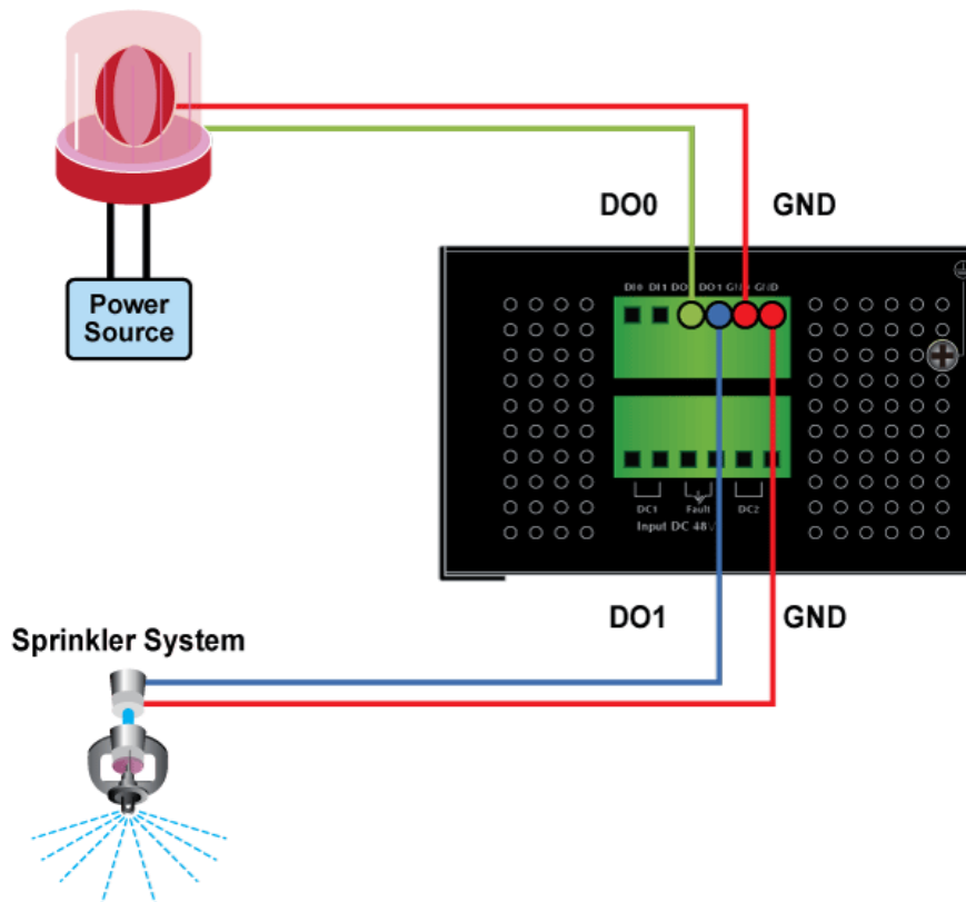
Figure 2-1-7d Wiring DO0 and DO1 to Open Detector
