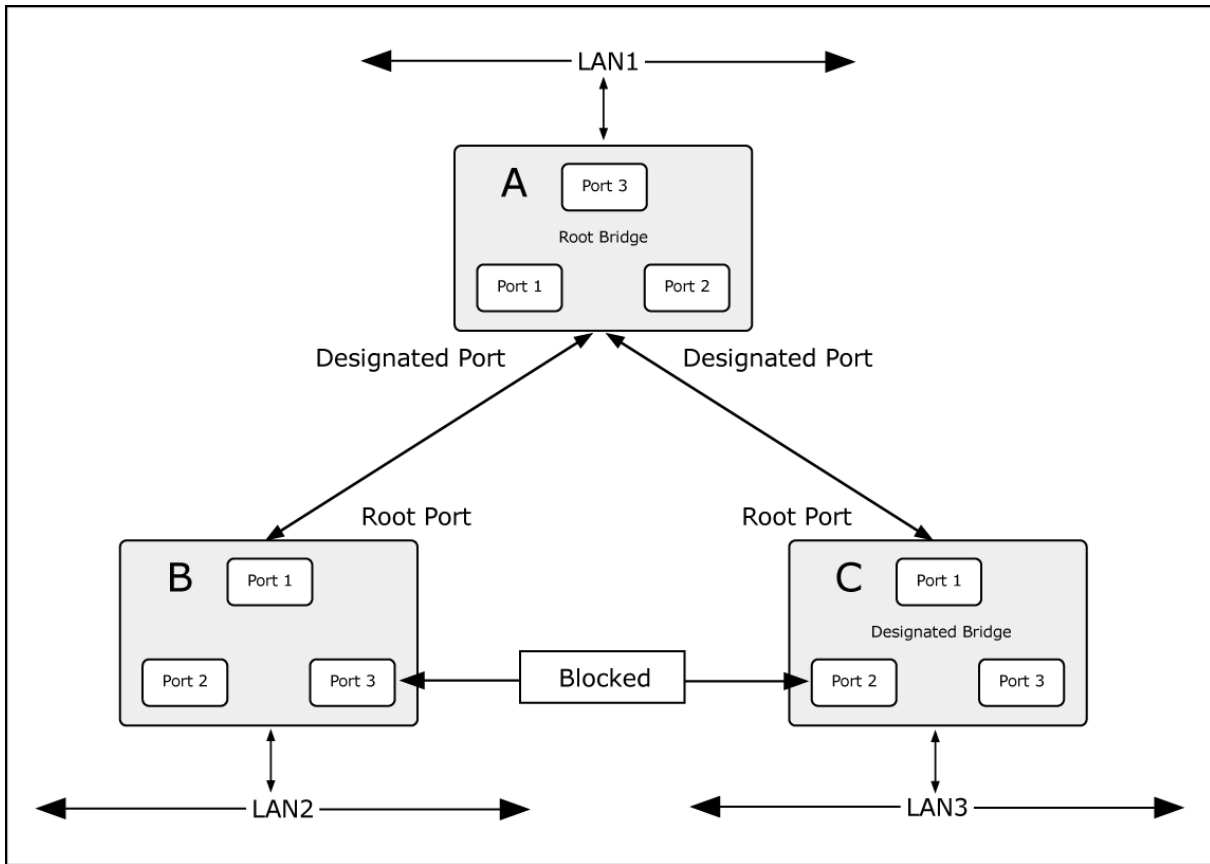
Figure 4-3-59 After Applying the STA Rules
