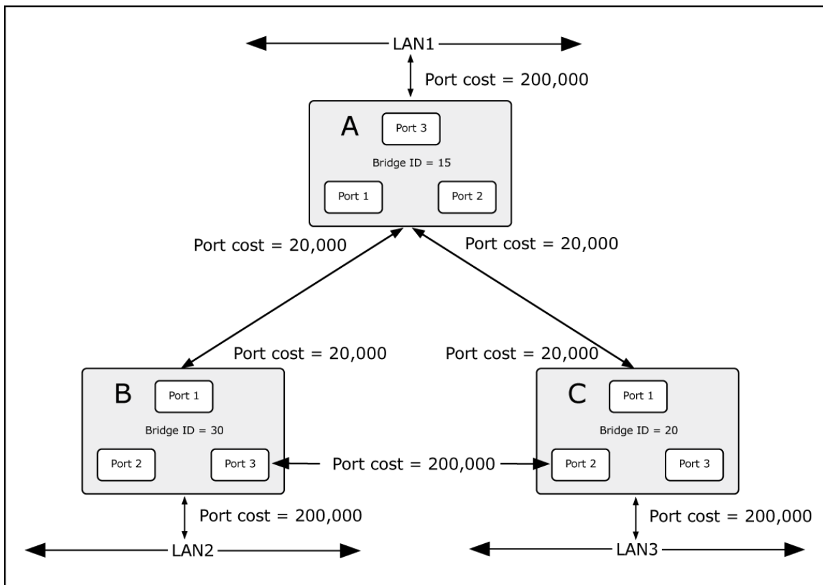
Figure 4-3-58 Before Applying the STA Rules
