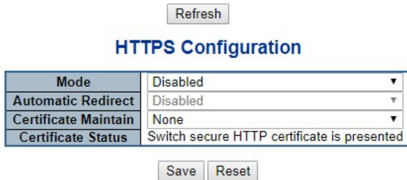
Figure 4-5-1-5: HTTPS Configuration Screen Page Screenshot
