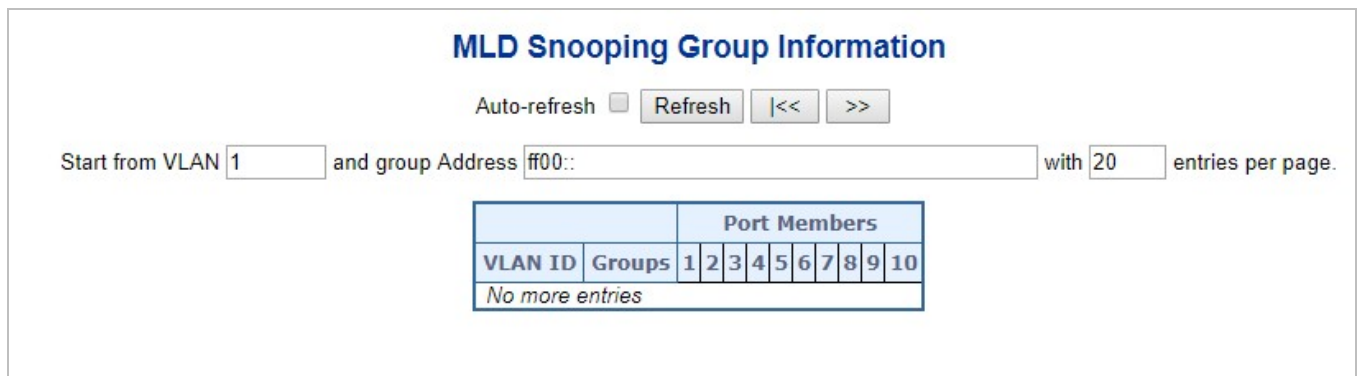
Figure 4-3-6-5: MLD Snooping Groups Information Page Screenshot
