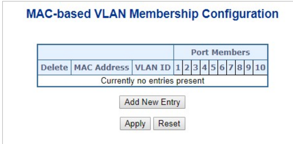
Figure 4-3-3-18: MAC-based VLAN Membership Configuration Page Screenshot
