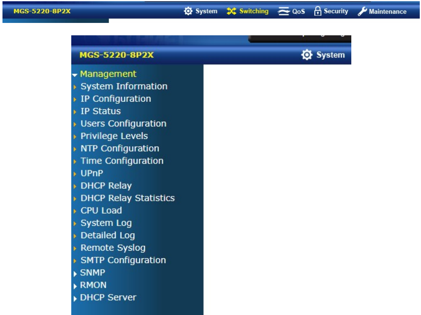
Figure 4-1-5: Managed Switch Main Functions Menu
