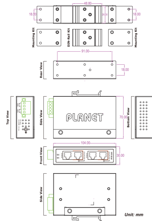
Figure 5: IPOE-260 Three-View Diagram
