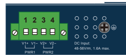
Figure 3: IPOE-260 Top View
