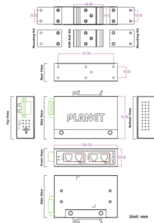
Figure 6: IPOE-260-12V Three-View Diagram
