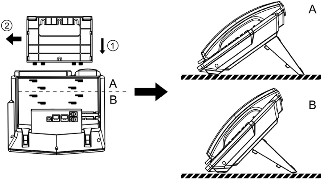
Figure 3 - Desktop Installation
