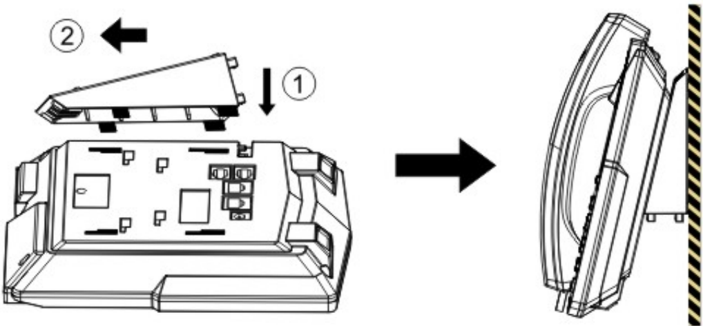
Figure 4 - Wall-mount Installation
