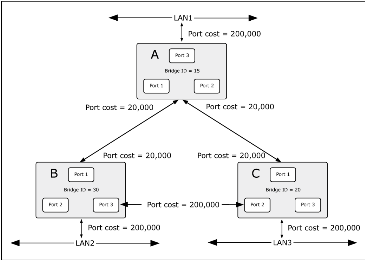
Figure 4-3-5-2: Before Applying the STA Rules
