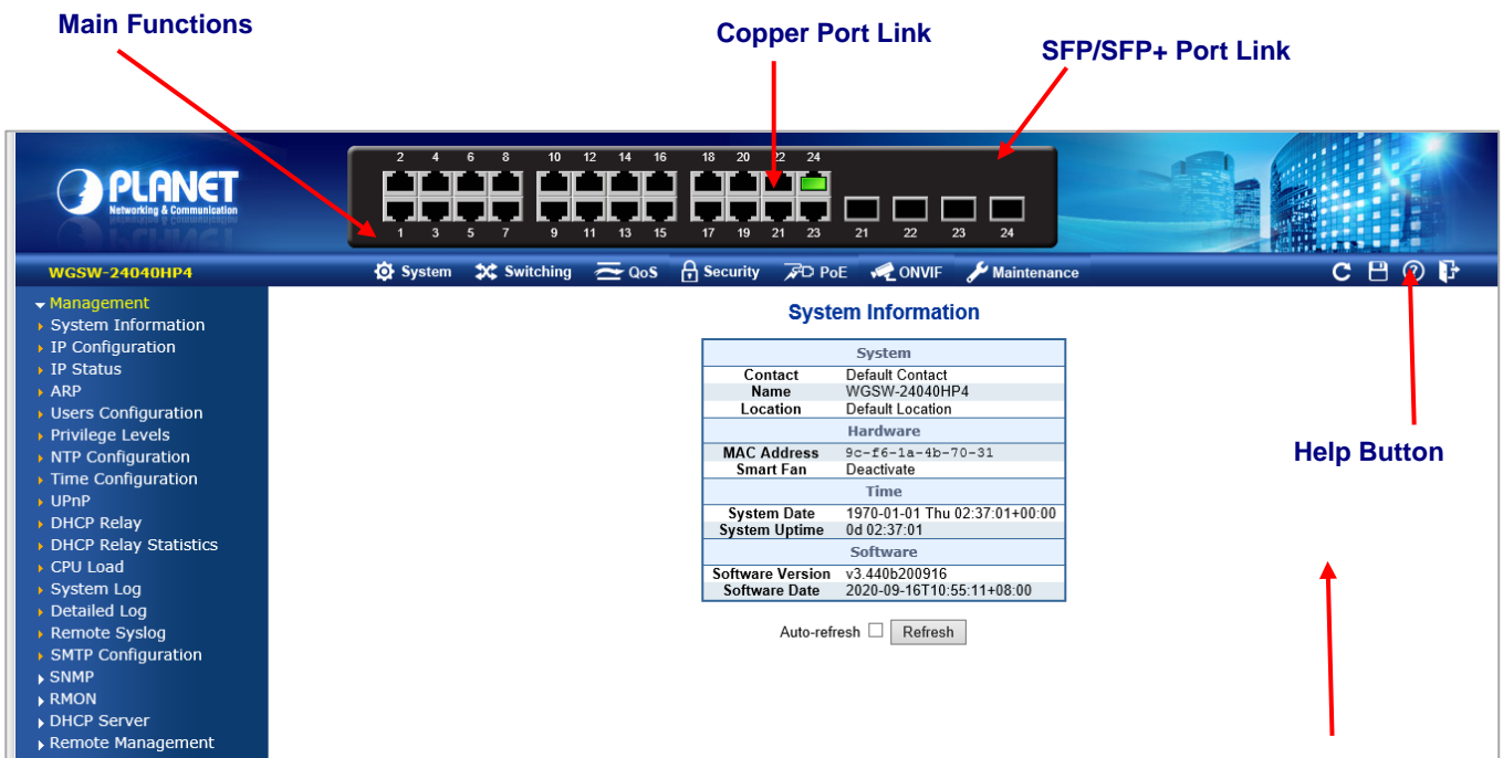
Figure 4-1-4: Web Main Page
