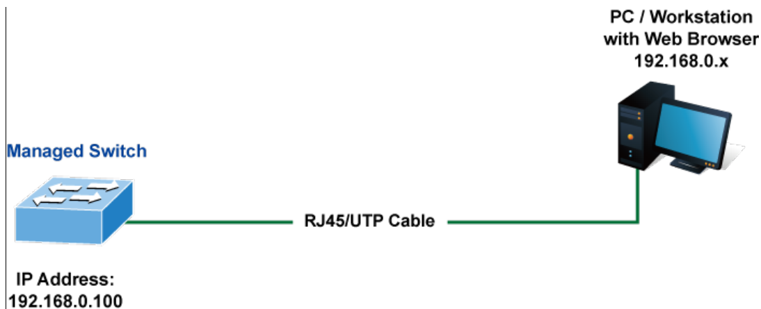
Figure 4-1-1: Web Management
