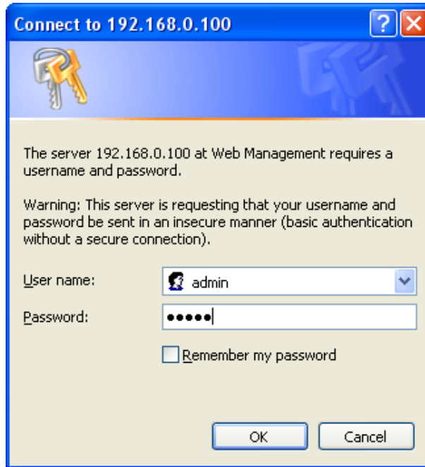
Figure 4-1-2: Login Screen
