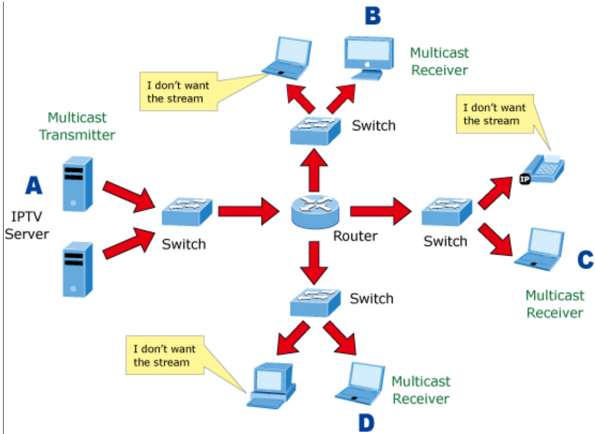
Figure 4-3-6-2: Multicast Flooding
