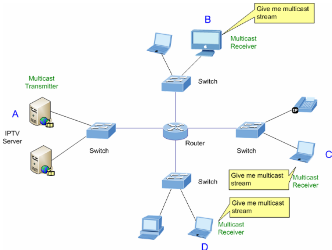
Figure 4-3-6-1: Multicast Service
