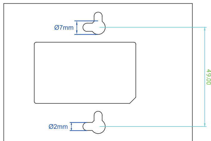
VC-231G/VC-231GF Switch Bottom Side
