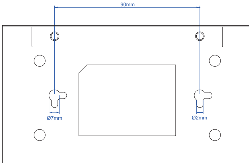
VC-234G Switch Bottom Side
