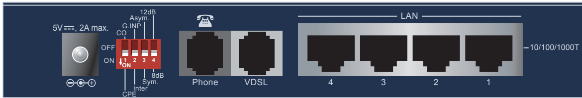
Figure 3-2-2: VC-234G Rear Panel
