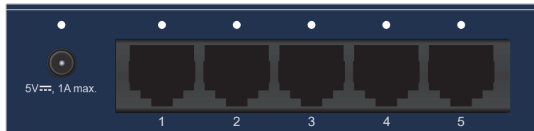
Figure 3-1: GSD-503 Front Panel
