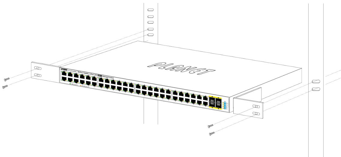
Figure 2-2-3: Mounting Managed Switch in a Rack
