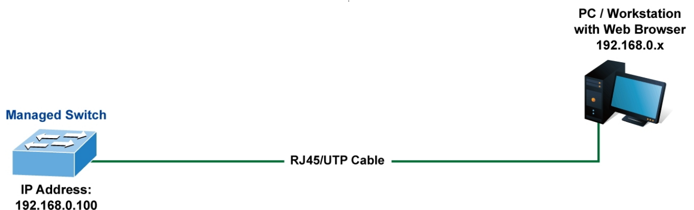
Figure 4-1-1: Web Management
