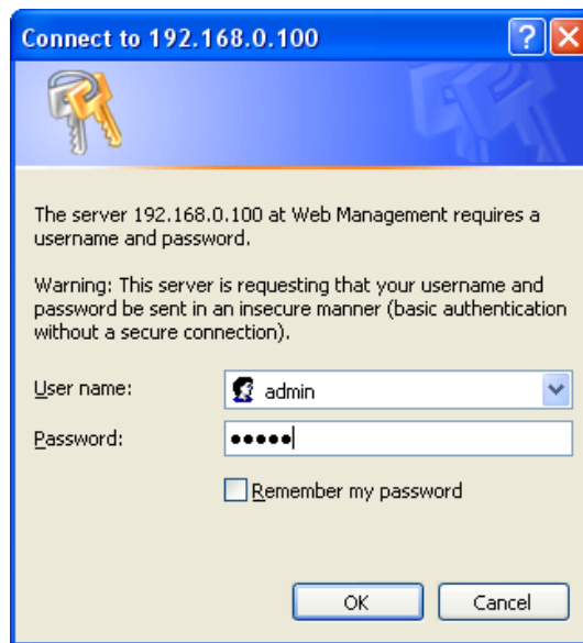
Figure 4-1-2: Login Screen
