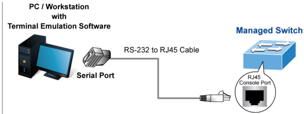
Figure 3-1-1: Console Management
