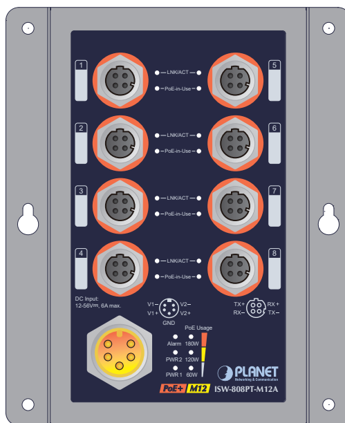
Figure 2-2: ISW-808PT-M12A Front Panel
