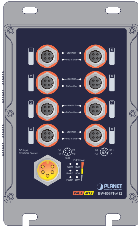
Figure 2-1: ISW-808PT-M12 Front Panel
