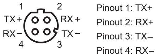
4-pin M12 Female 10/100TX Connector Pin Assignment
