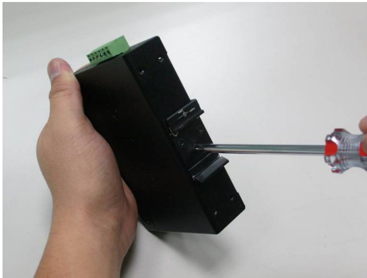
Step 1: screw the DIN-Rail on the Industrial Managed Media Converter.
