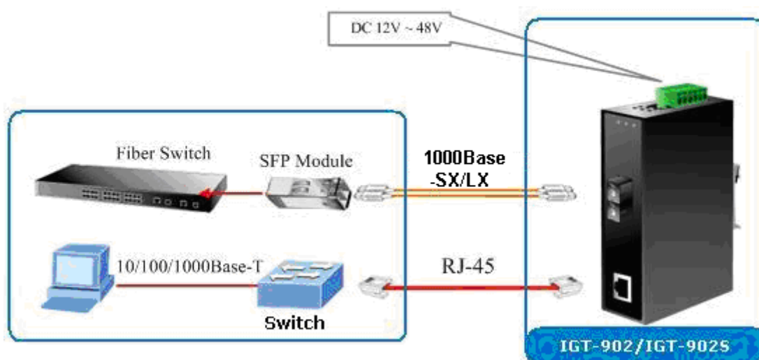
Figure 2-7 IGT- 902 / IGT-902T / IGT-902S / IGT-902TS stand-alone installation
