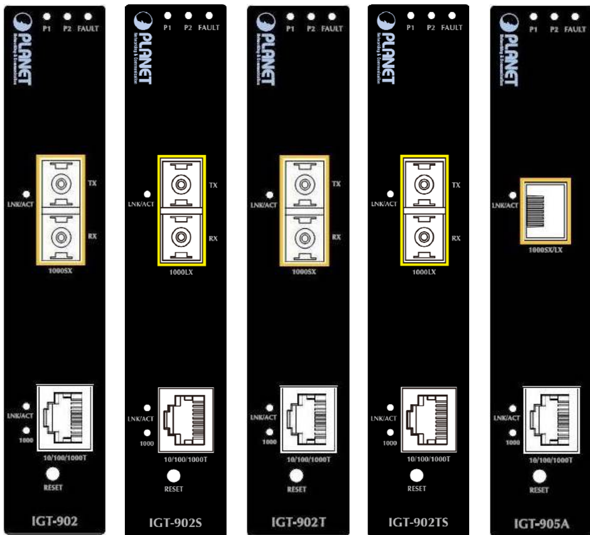
Figure 2-1 & 2-2 PLANET IGT-902 / IGT-902S Front Panel
