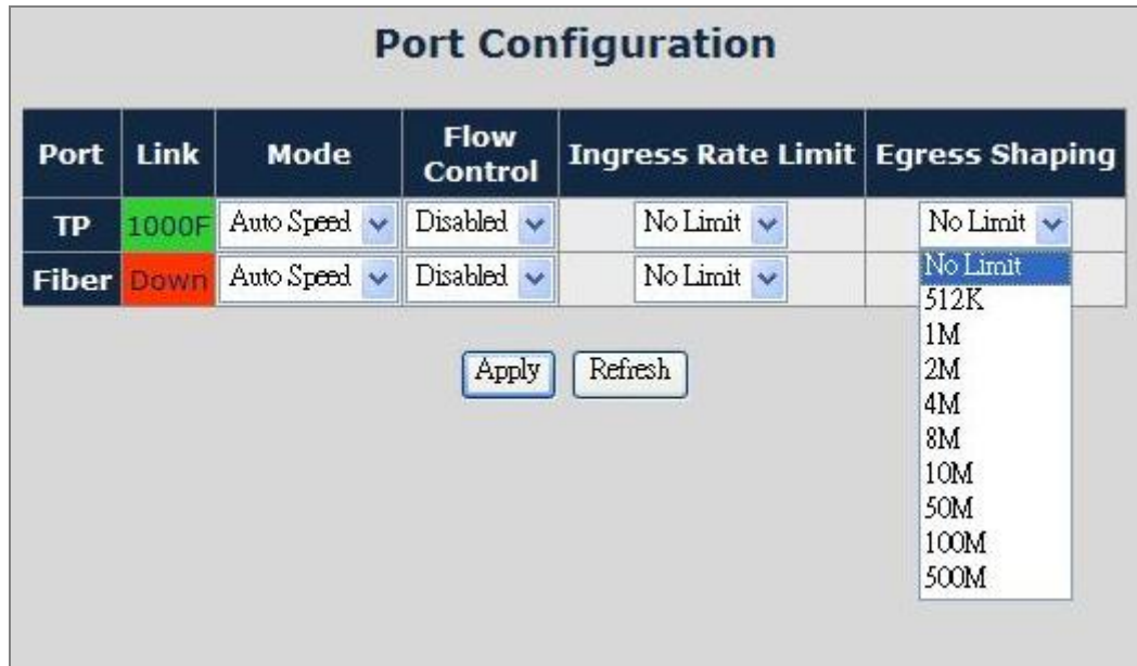
Figure 4-22 Port Configuration-Egress Shaping Web Page screen
