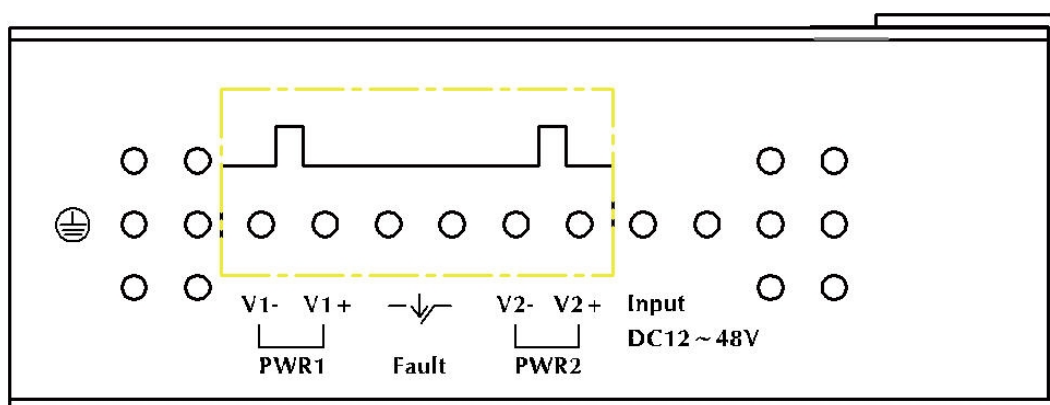
Figure 2-6 Upper Panel of IGT-90X
