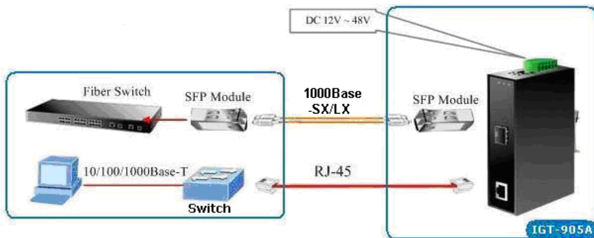
Figure 2-8 IGT- 905A stand alone installation
