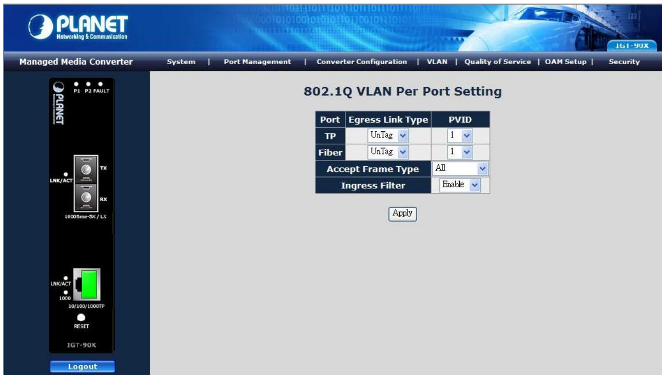
Figure 4-28 VLAN Per Port Setting Web Page screen
