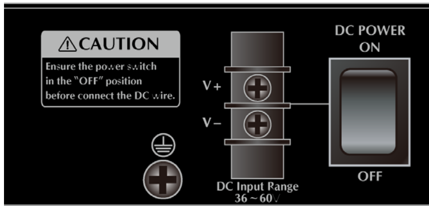
Figure 2-1-7 Rear Panel of WS redundant power model
