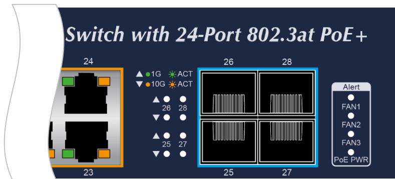
Figure 2-1-5: WS-2864PVR LEDs on Front Panel
