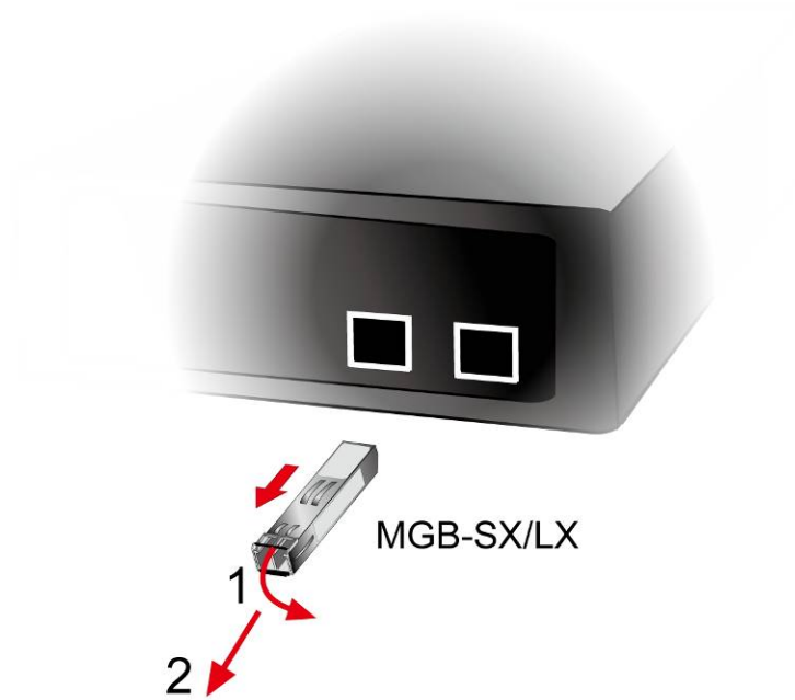
Figure 2-2-5: How to Pull Out the SFP/SFP+ Transceiver
