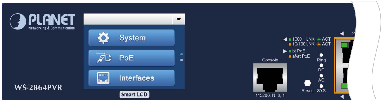
Figure 2-1-4: WS-2864PVR LEDs on Front Panel
