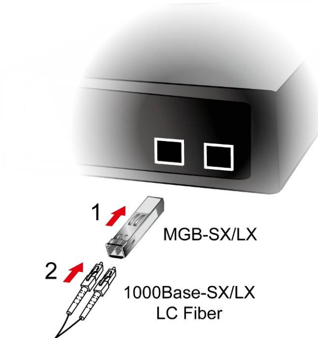
Figure 2-2-4: Plug-in the SFP/SFP+ Transceiver
