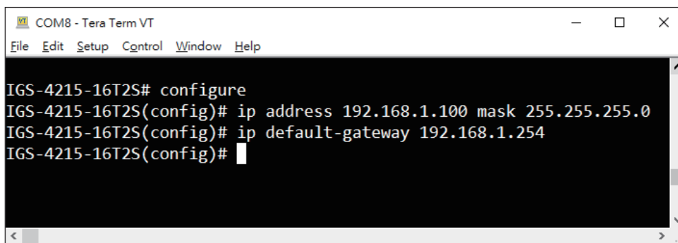
Figure 4-6: Configuring IP Address Screen
