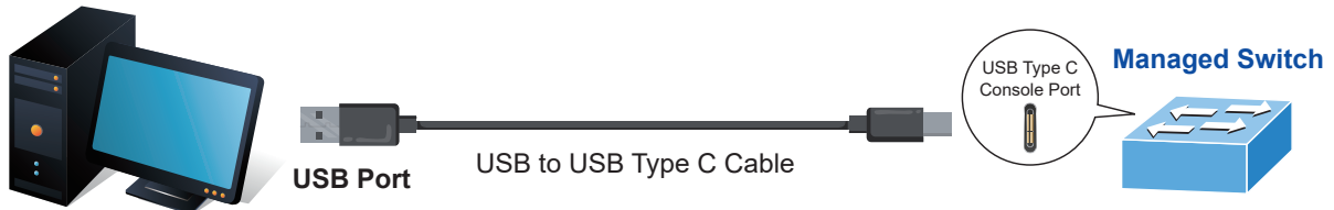
Figure 4-1: Industrial Managed Switch Console Connectivity
