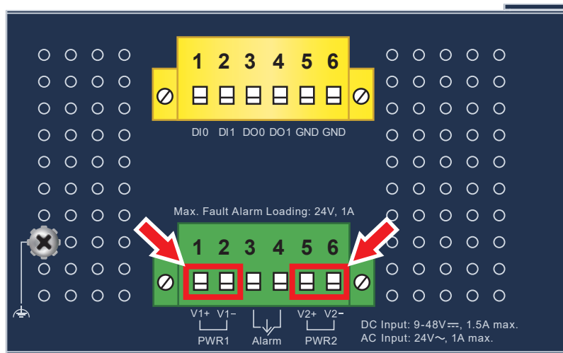
Figure 3-1: IGS-4215-16T2S Inlet Power Socket
