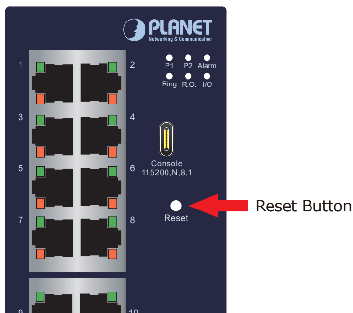
Figure 6-1: Reset Button
