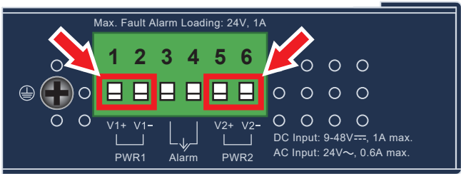
Figure 3-3: IGS-4215-4T2S Inlet Power Socket
