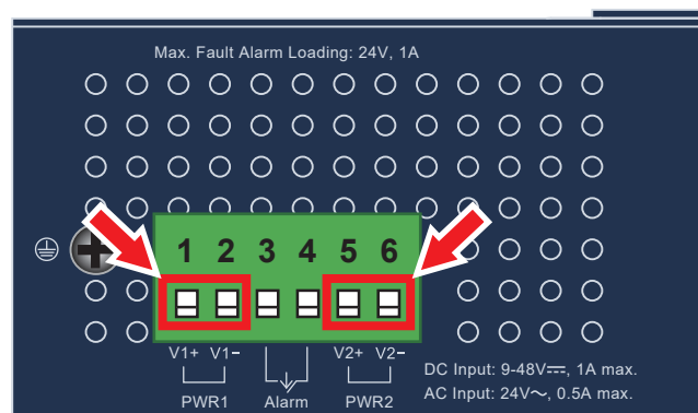
Figure 3-2: IGS-4215-8T2S Inlet Power Socket
