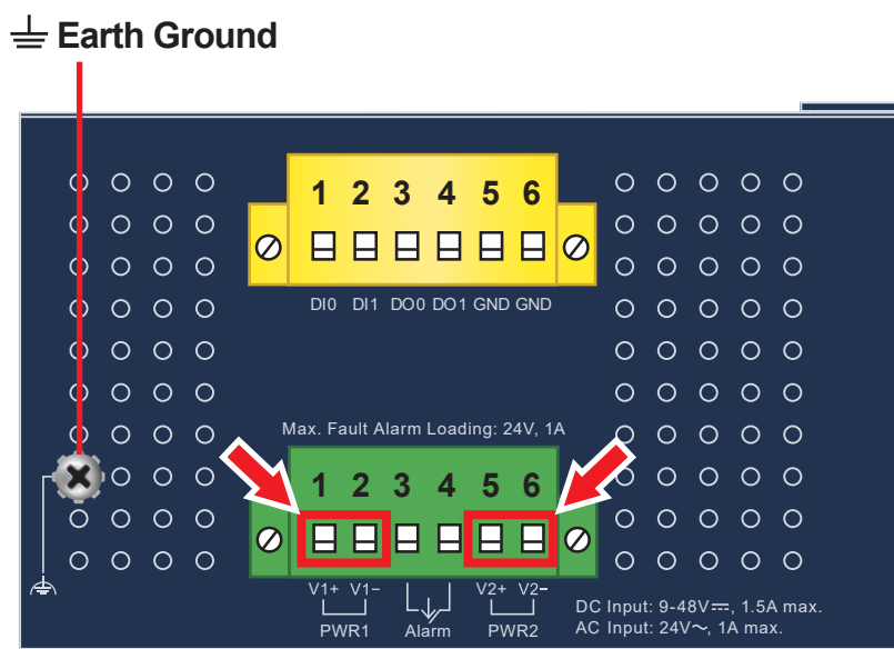
Figure 3-4: Grounding Method (applies to all models)
